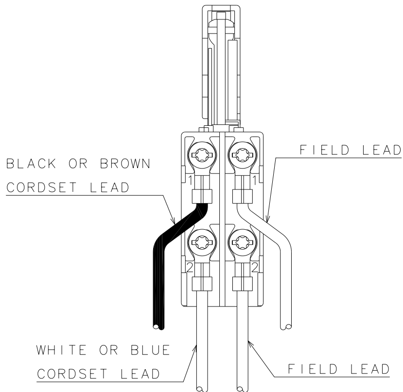
120V/220V SWITCH CONNECTION VIEW
