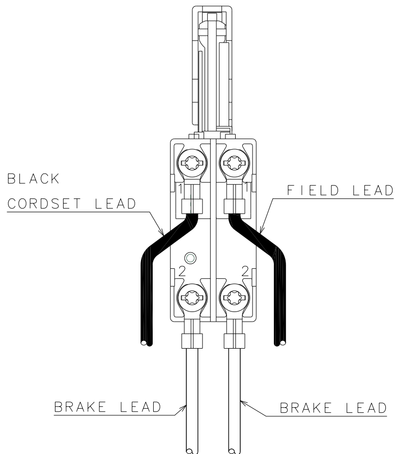
120V BRAKE UNIT SWITCH CONNECTION VIEW
