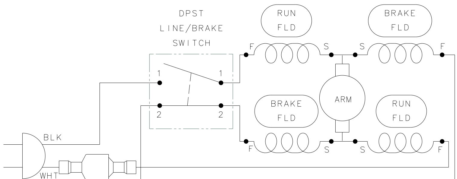
120V BRAKE UNIT WIRING SCHEMATIC
